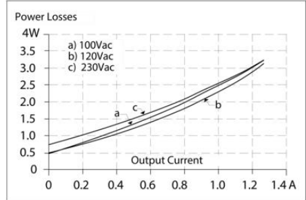
Fig. 8-2 Losses vs. output current at 12V, typ.
